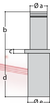
DAMPY B Ø219/500-700 DAMPY B Ø219/500-700 S/STEEL
